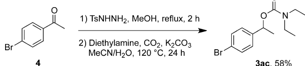
Scheme 3. One-pot synthesis of 3ac . Reaction conditions: 1) 4 (0.5 mmol), tosylhydrazide (0.5 mmol), reflux, 2 h; 2) diethylamine (5 mmol), K_2CO_3 (1.5 mmol), CO_2 (4 MPa), MeCN/ H_2O (3 mL, 15:1 v/v), 120 °C, 24 h.
